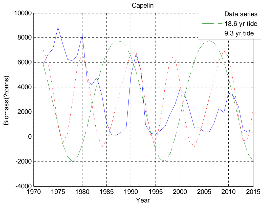
Figure 7. Barents Sea capelin biomass from 1972 to 2005, with the biomass prediction from 2005 to 2015, the astronomic 18.6 yr tide cycle and the 9.3 yr tide cycle.
