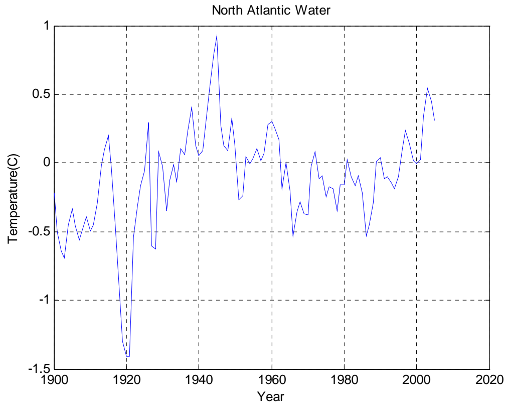
Figure 2. The North Atlantic data series from 1900 to 2005.
