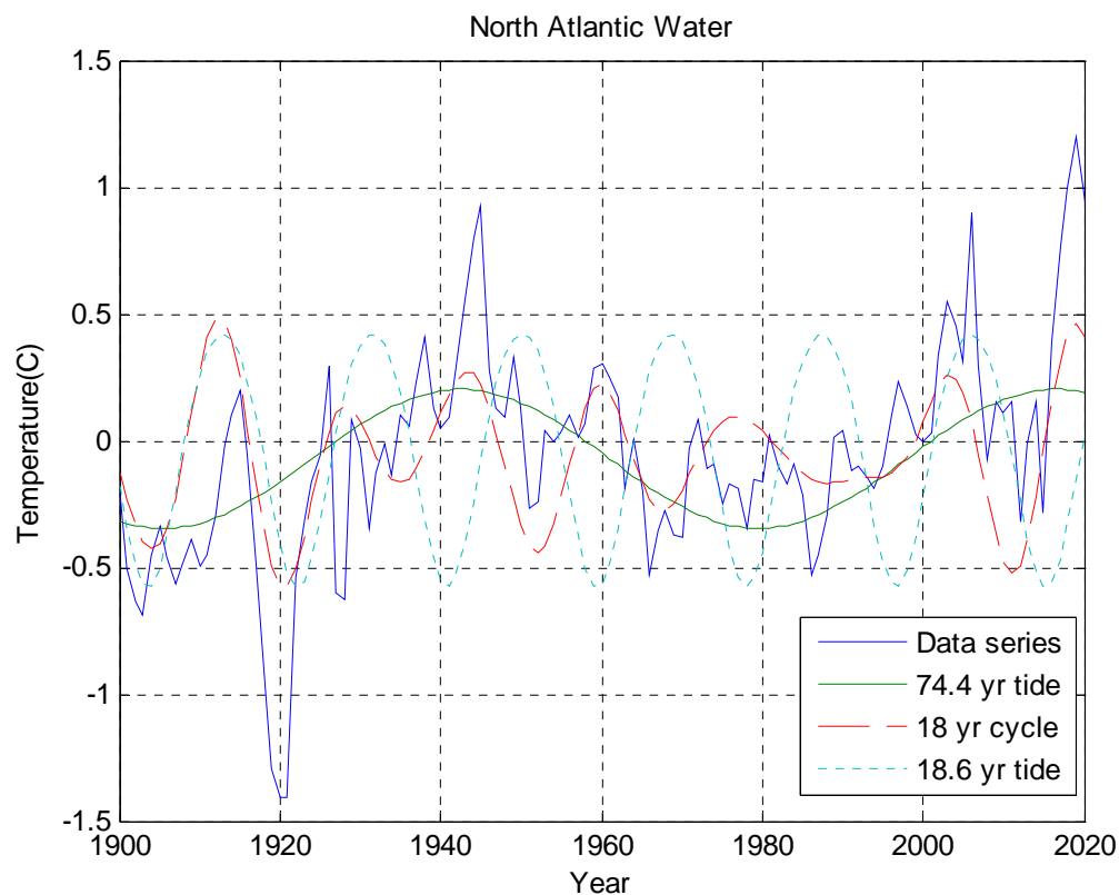
Figure 3. North Atlantic Water temperature from 1900 to 2005 and temperature predictions from 2005 to 2020. The estimated 74.4 yr tide cycle, the identified 18 yr wavelet cycle and the 18.6 yr tide cycle are also shown.
