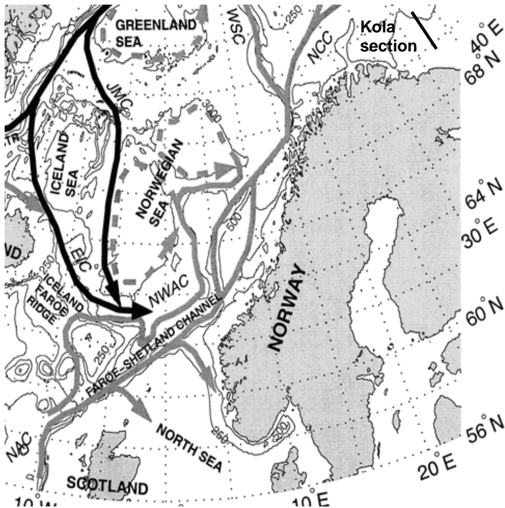
Figure 1. Currents in the Faroe-Shetland channel and the Kola section.
