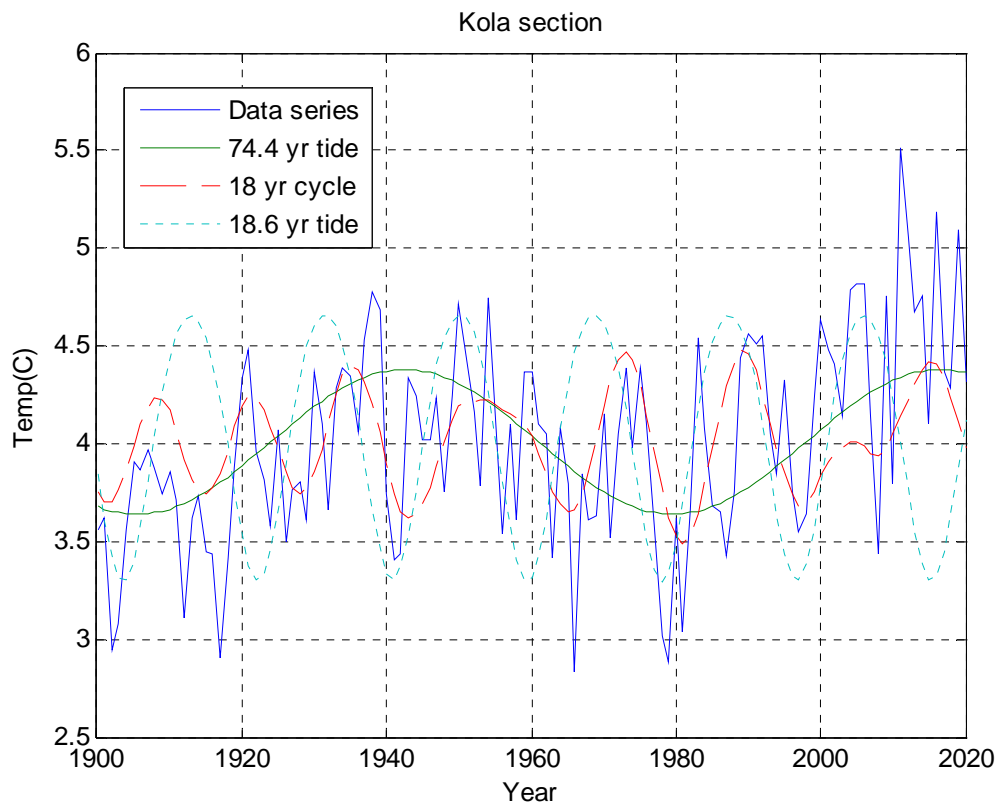
Figure 4. Temperature series from 1900 to 2005, temperature forecast to 2020, the 18.6 yr tide, the 74,4 yr tide and the identified 18 yr cycle are shown for the Kola section of the Barents Sea.
