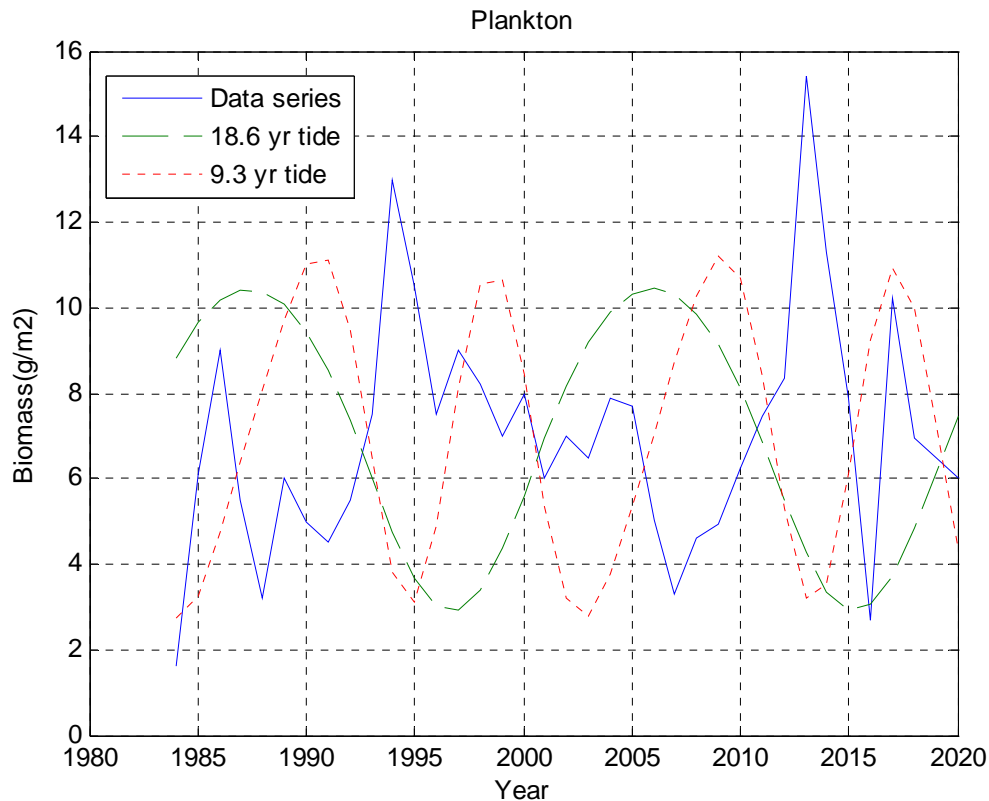
Figure 5. Barents Sea zooplankton dry weight biomass data series from 1984 to 2005 is shown, along with the biomass prediction from 2005 to 2020, the astronomic 18.6 yr amplitude tide, and the 9.3 yr phase tide.
